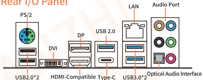
1-2 Overall Rear I/O Panel Display
