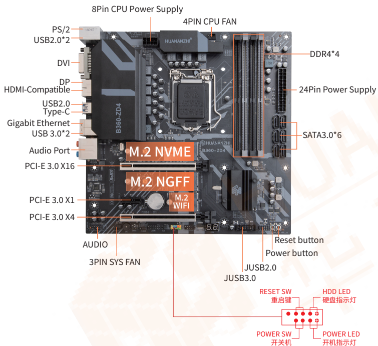
1-1 B360-ZD4 Motherboard Illustration
